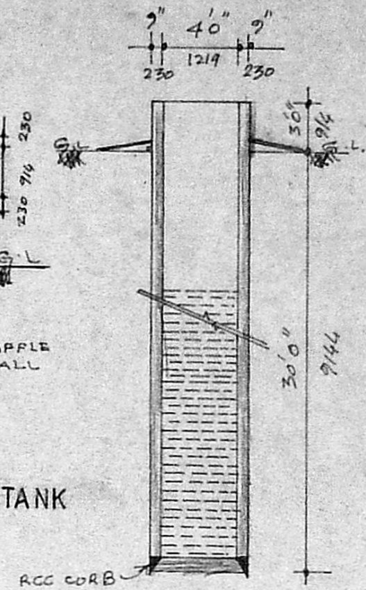
DETAIL OF 4-0 (1219) DIA WELL
